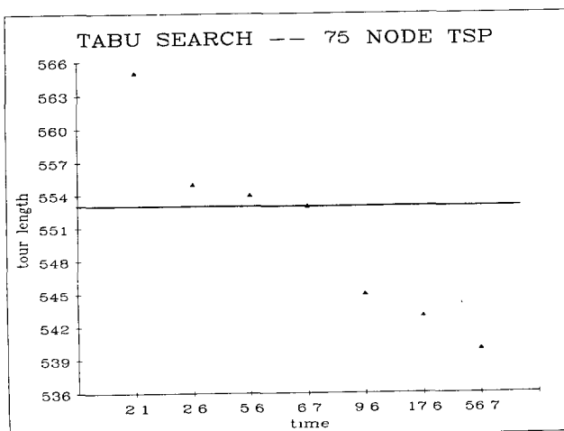
Figure 1. Typical run for 75 node problem.
