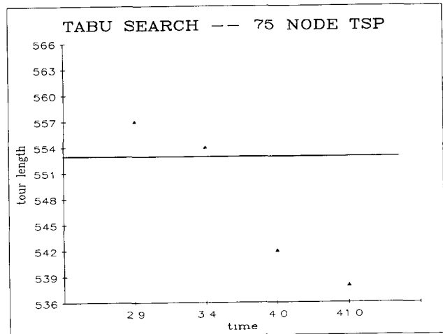
Figure 2. Typical run for 75 node problem.
